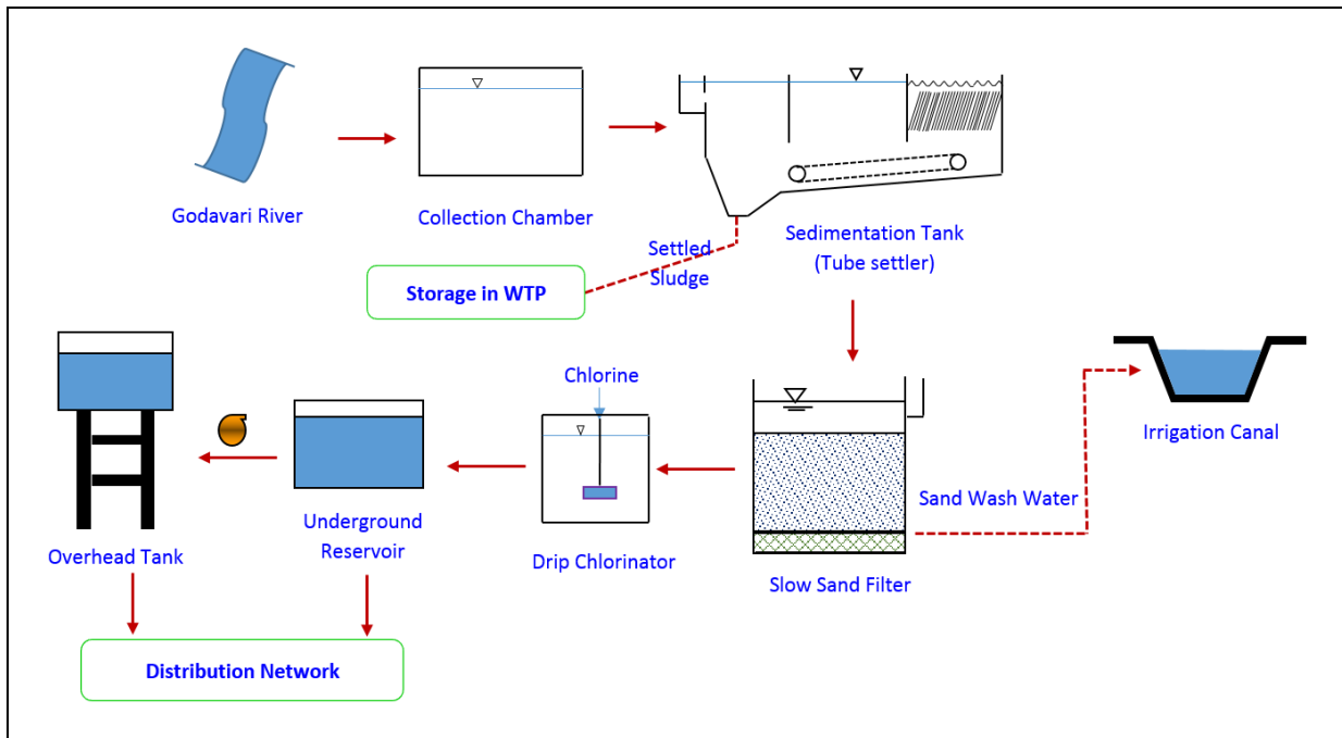
Figure 1: Schematic Diagram of Water Treatment Processes
